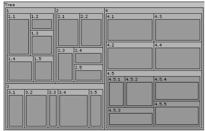
Figure 3: Labeled Treemaps.
